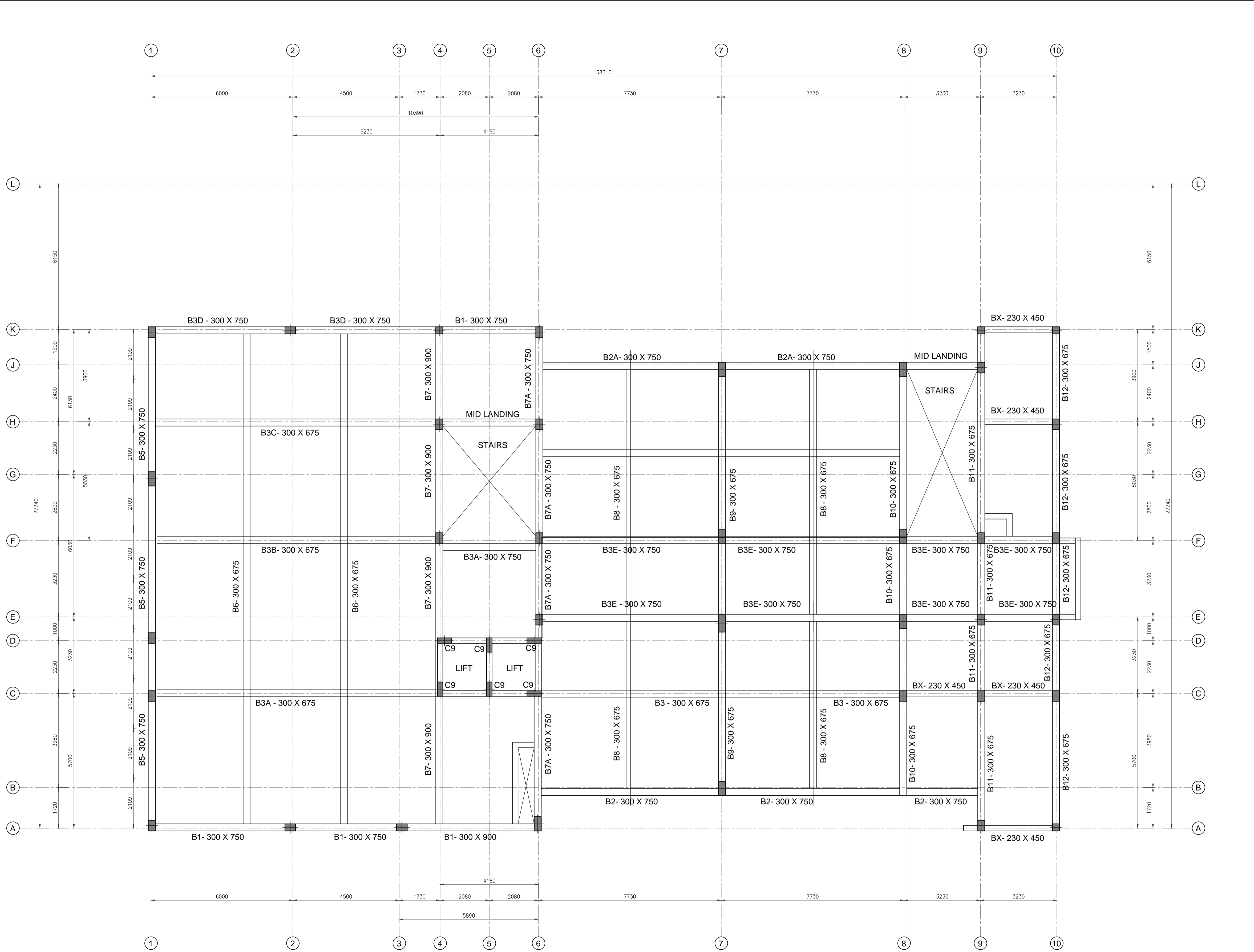
TERRACE FLOOR LVL BEAM LAYOUT ALL SLABS ARE 140 THK
